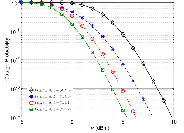
Fig. 5. Outage probability of the C-MRT technique for various locations of relays when N = 3 and K_i = 3 for all i \in \mathcal{R} .
